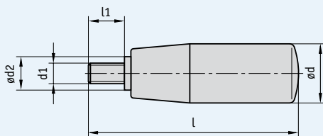
Cylindric handle
