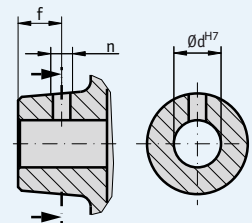
hub thread
