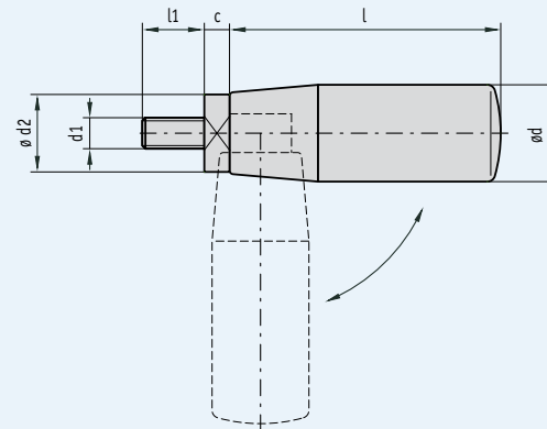
Fold-away handle
