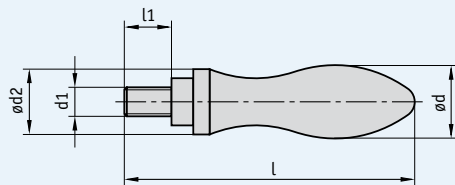
Cylindric handle
